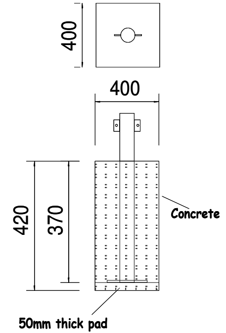
1m Posts Front Post Installation Detail
