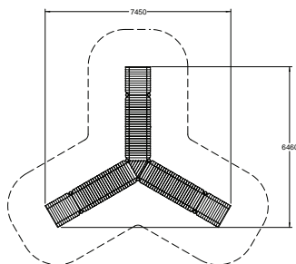
Concave and convex timber boardwalks
